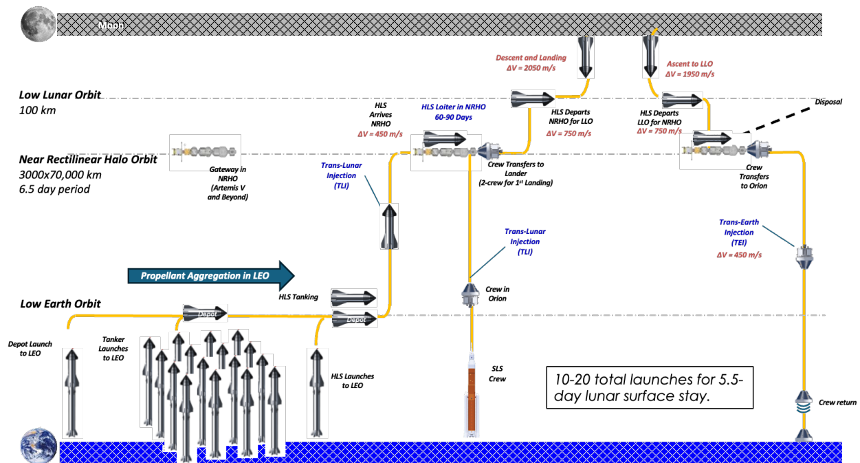
Fig. 5. Artemis III Concept of Operations
