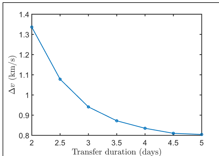
Fig. 10. \Delta V vs. Trip Time for Departure from 100 km Circular Lunar Orbit 32
