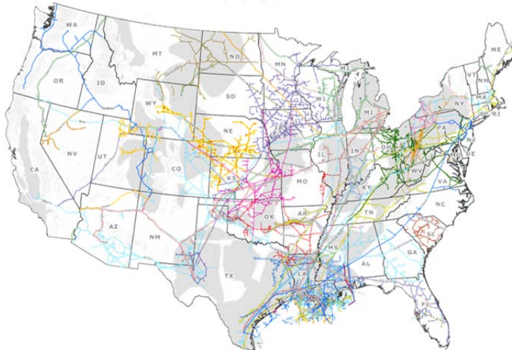
U.S. Interstate Natural Gas Transmission Pipelines
