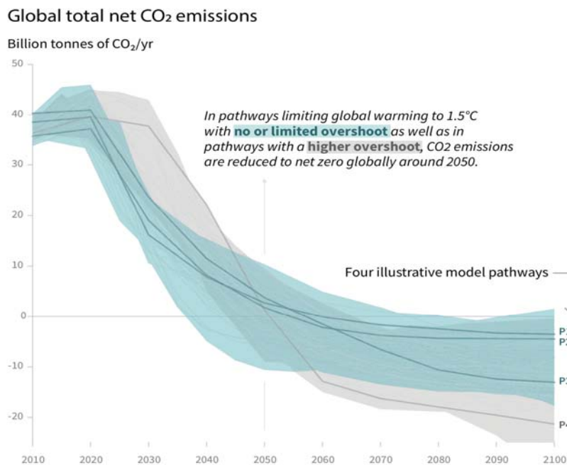
Figure 1: Pathways to limit global temperature to the Paris Agreement target of no more than 1.5 degree warming (Source: IPCC, Special Report: Global warming of 1.5 o C, 2018)
