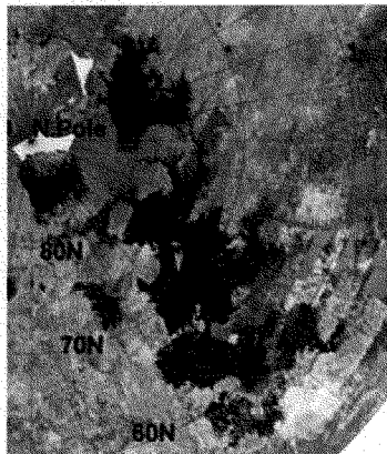
Figure 3 (credit NASA/JPL-Caltech/USGS)
