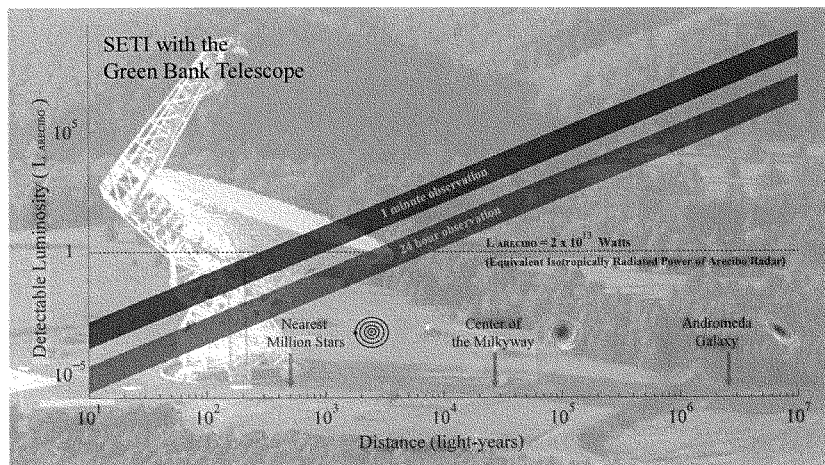
Figure 6: The sensitivity of the Green Bank Telescope expressed as the luminosity detectable as a function of the transmitter distance. Both 1 minute and 24 hour observation durations are indicated. The detectable luminosity is indicated in units of the luminosity of the Arecibo Planetary Radar – the most powerful radio transmitter on Earth. As shown, the Green Bank Telescope could detect a radio transmitter with the same luminosity as the Arecibo Planetary Radar, in 1 minute each, for more than 1 million nearby stars.
