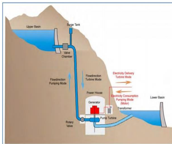
Figure 1 Typical Pumped Storage Facility. Source: Alstom Power
