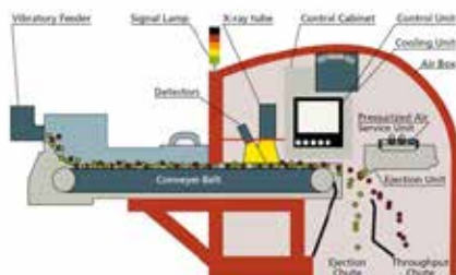
Figure 27. Redwave XRF-based plastic separator. Source: Redwave Austria
