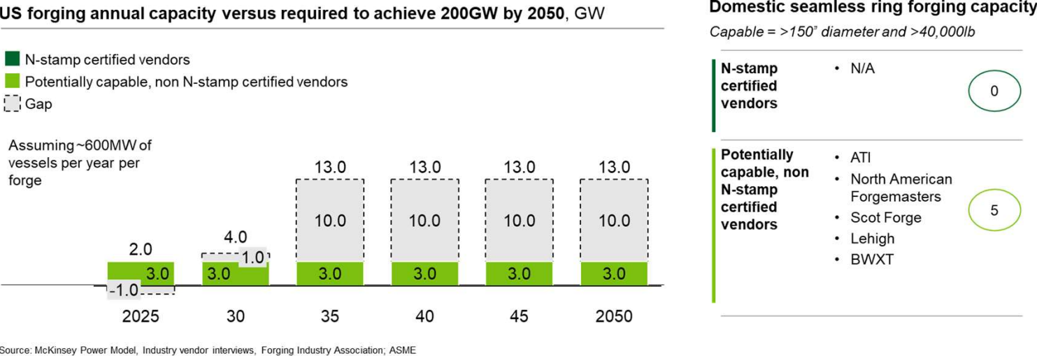
Figure 28: U.S. ring-forging capacity to achieve 200 GW by 2050 versus existing capacity, assuming all designs required ring forging
