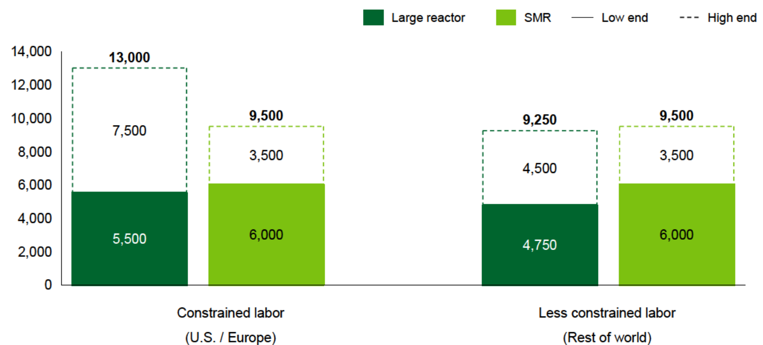
Figure 19: Overnight capital costs of large and small reactors by labor environment xxxi
