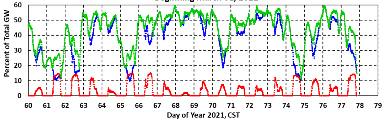
ERCOT Wind, Solar, (Wind + Solar) Generation (Percent of Total), Beginning March 01, 2021
