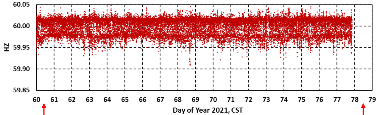
ERCOT Frequency, Beginning March 01, 2021
